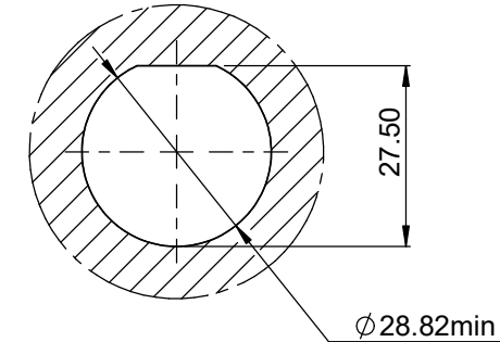
MOUNTING PANEL CUT
